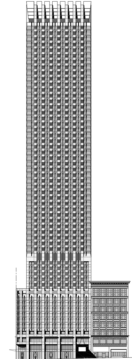
East elevation
